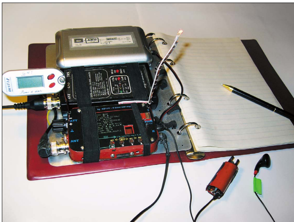
Portable set by Pavel, OK1MN: ATS-3B1 TCVR, Elecraft T-1 antenna tuner, solar cells, clock, LED light, mini paddle
